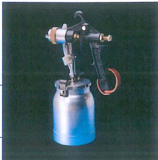
#880 1Quart Cup Hand Spray Gun
